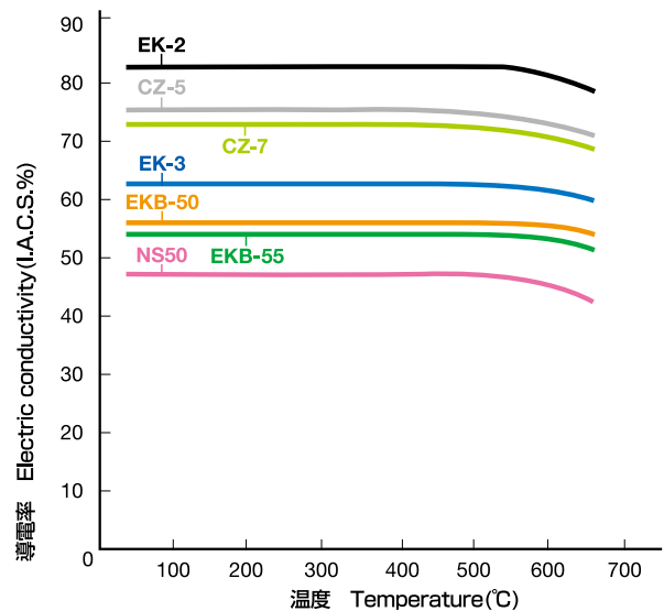
高温熱処理後の導電率の変化 Room temperature electric conductivity after one hour holding in high temperature
